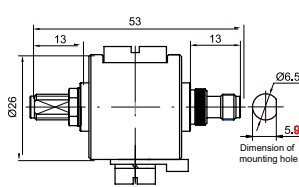
P8AX_-SMA/FF
