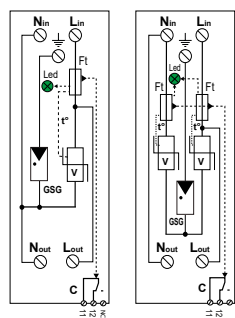
DACN10S-L11-xxx DACN10S-L21YG-275
