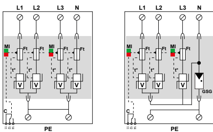
DAC15CS-40
