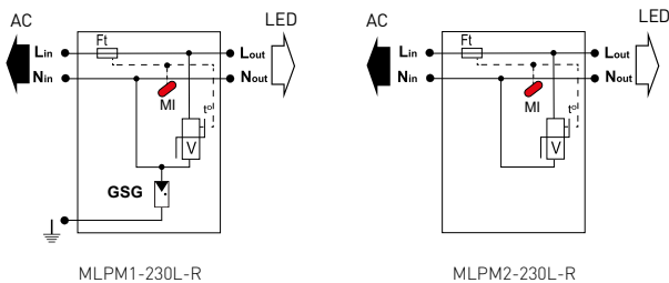
MLPM1-230L-R
