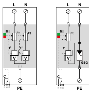
DAC15CS-20 DAC15CS-11
