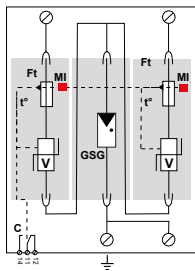
DS50PVS-800G/51 DS50PVS-1000G/51
