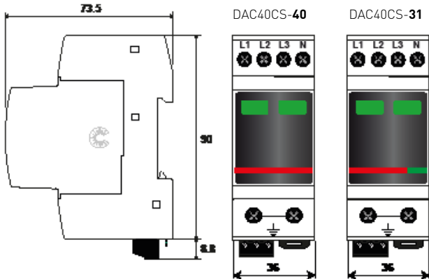
DAC40CS-40
