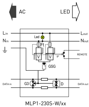
MLP1-230S-W/xx
