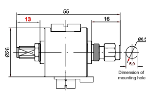
P8AX_-SMA/MF
