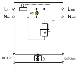
MLP2-230L-P/xx
