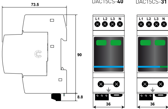
DAC15CS-40
